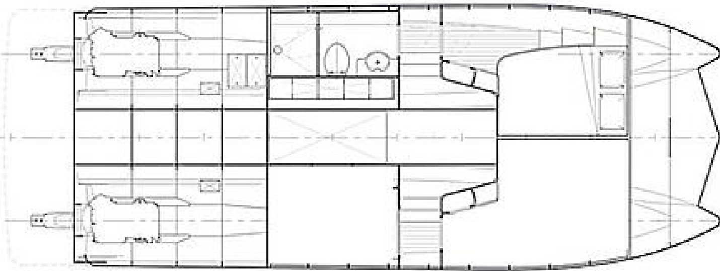
LOWER DECK LAYOUT
