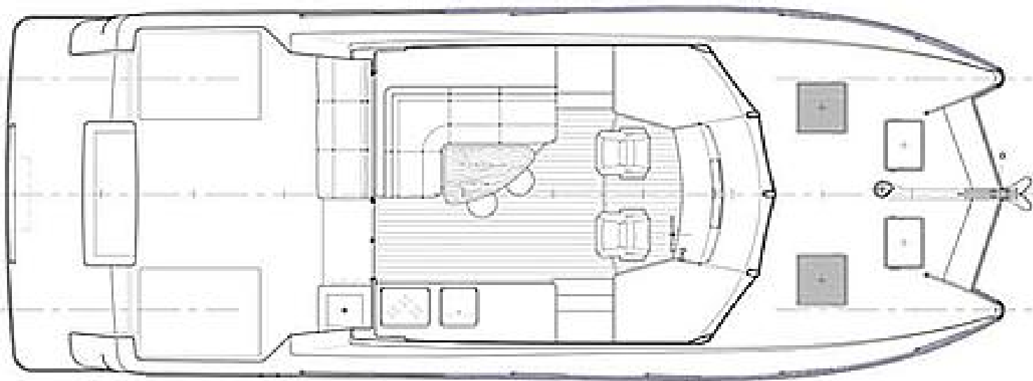
MAIN DECK LAYOUT
