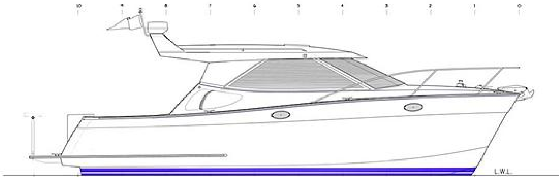
OUTBOARD PROFILE
